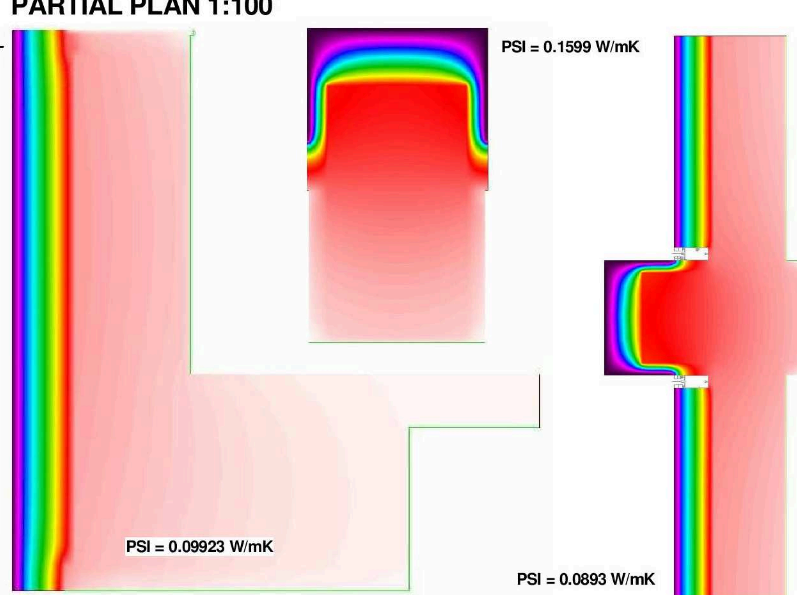
THERMAL BRIDGE ANALYSIS OF KEY JUNCTIONS
