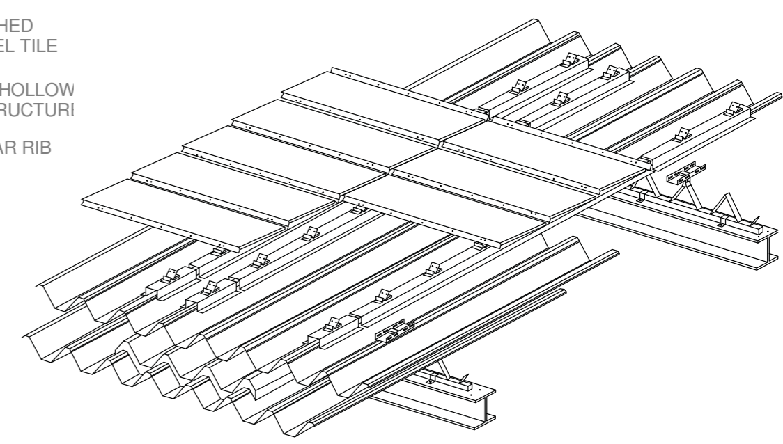
3D OF ROOF DETAIL 1:75
