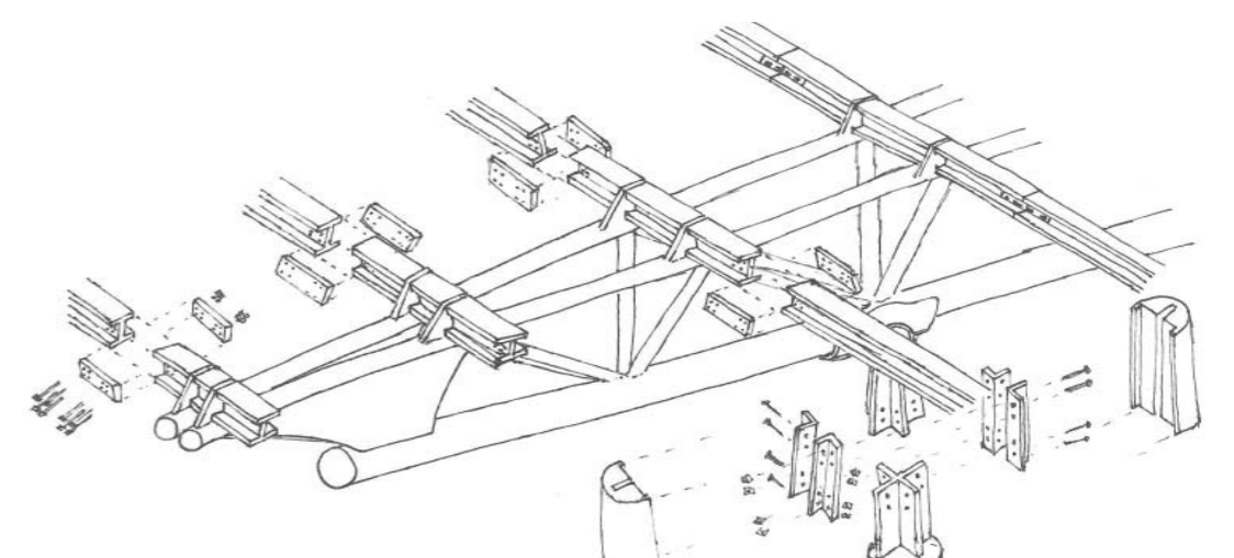
3D OF EAVE DETAIL 1:75
