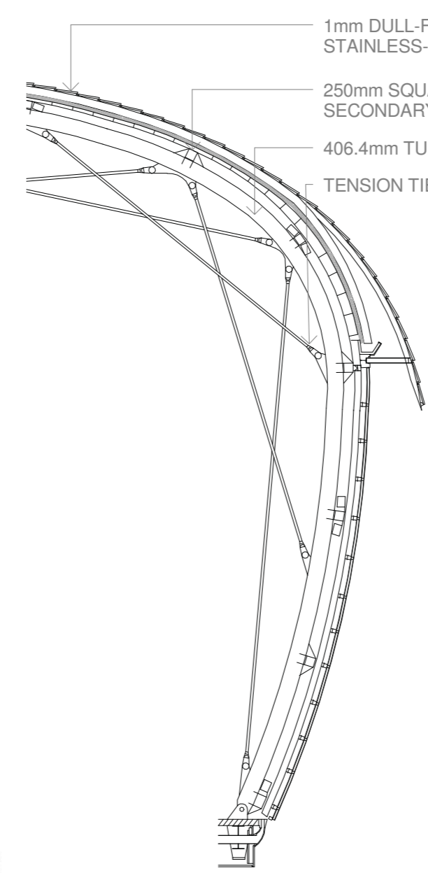
WING DETAIL 1:150
