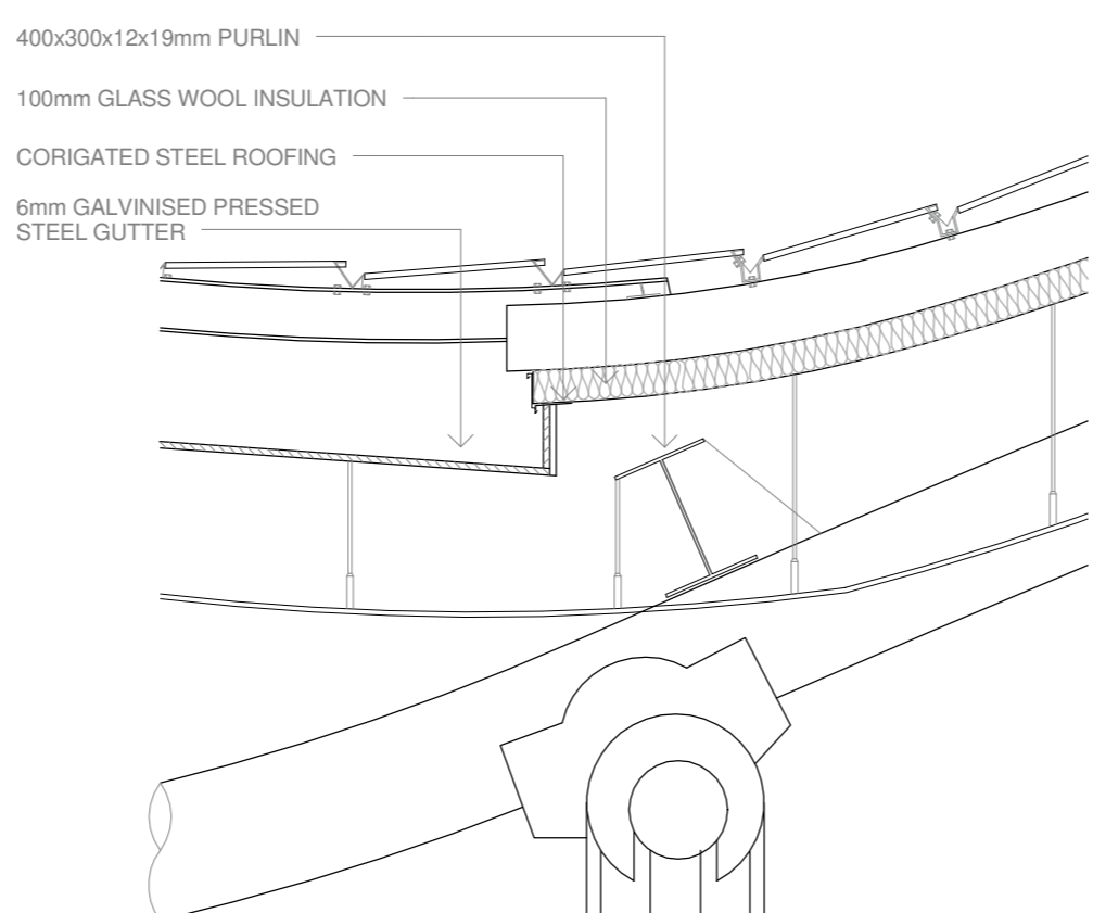
ROOF JUNCTION DETAIL 1:25
