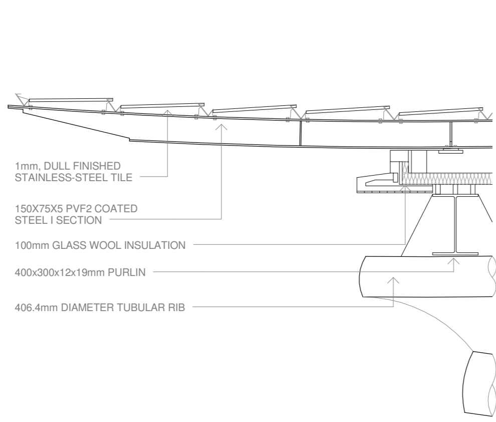
EAVES DETAIL 1:25
