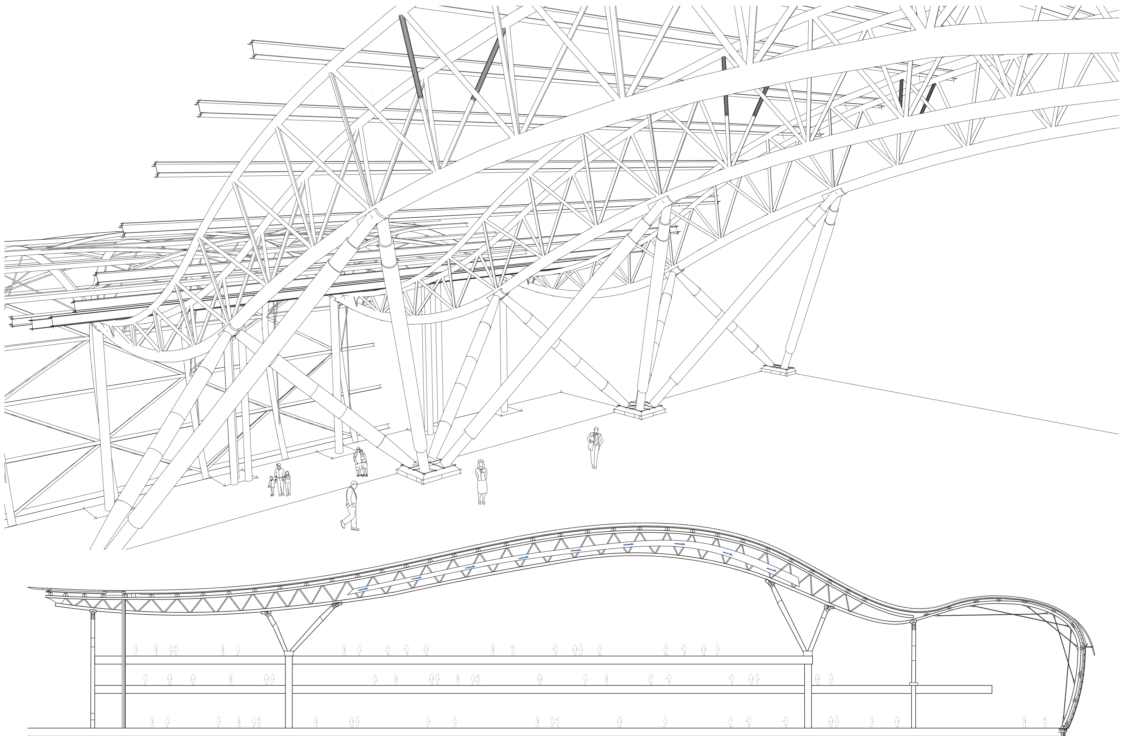
SECTION 1: 300
