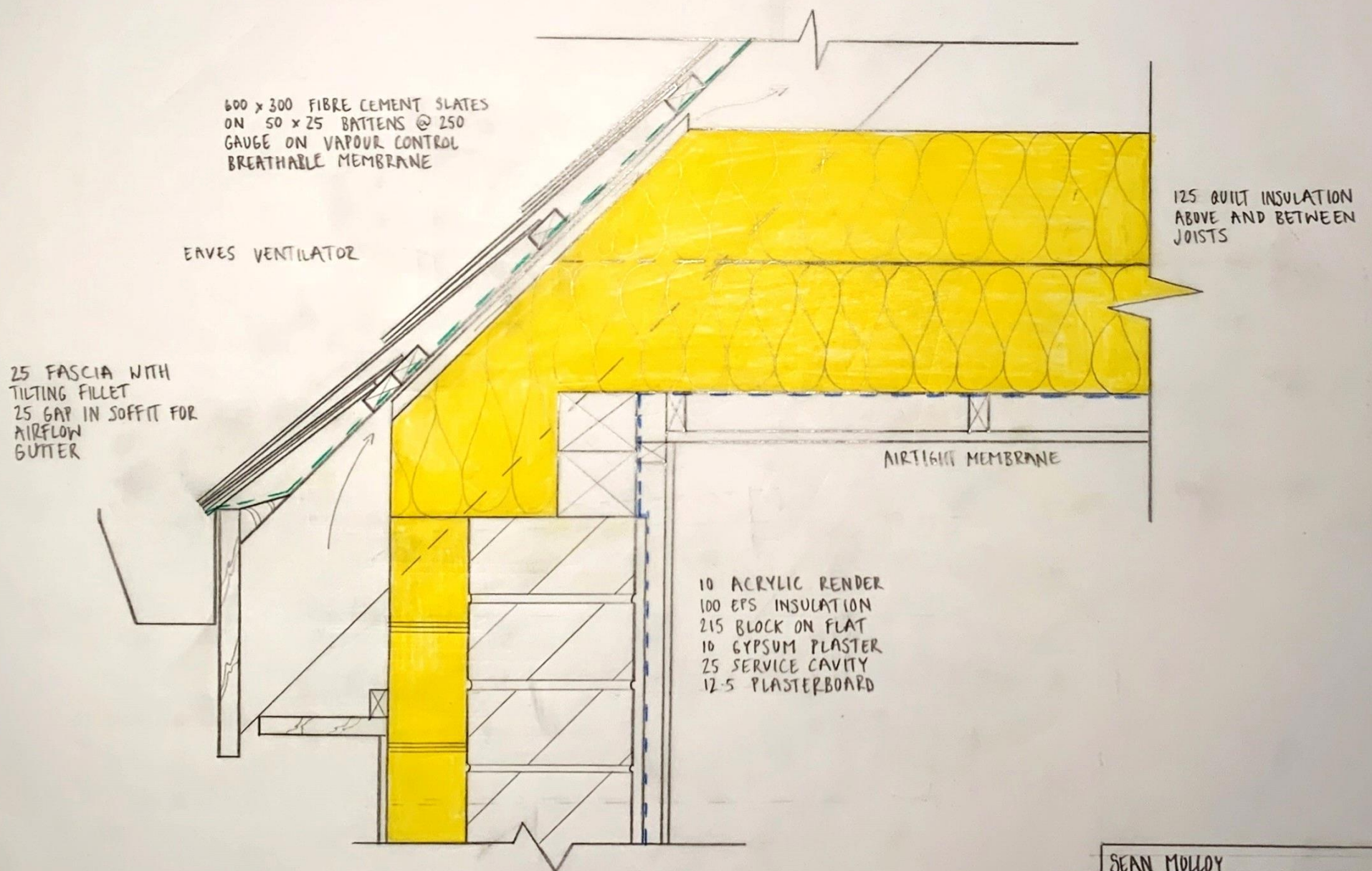
WALL TO ROOF EAVES DETAIL
